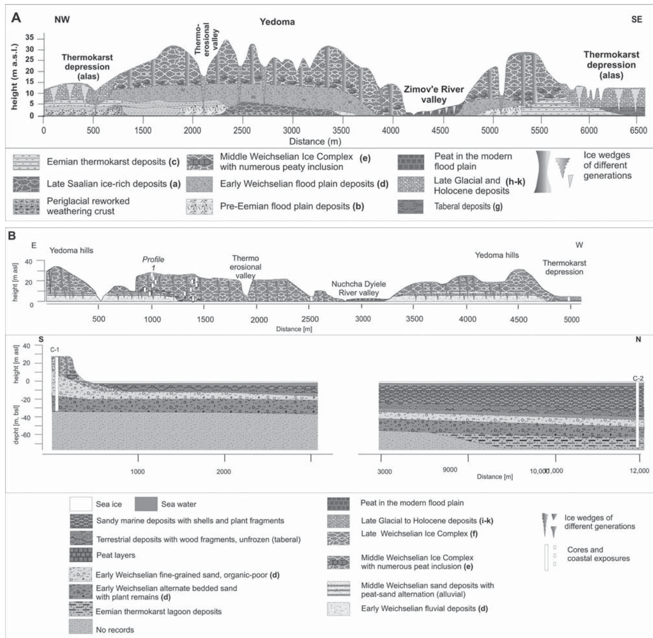
Figure 2. Schematic cross sections of exemplary permafrost sequences. (a) Section exposed at south coast of Bol'shoy Lyakhovskiy Island at the Dmitry Laptev Strait (site 17 in Figure 1). (b) Section and drilling transect at Cape Mamontov Klyk in the western Laptev Sea (site 1 in Figure 1).
