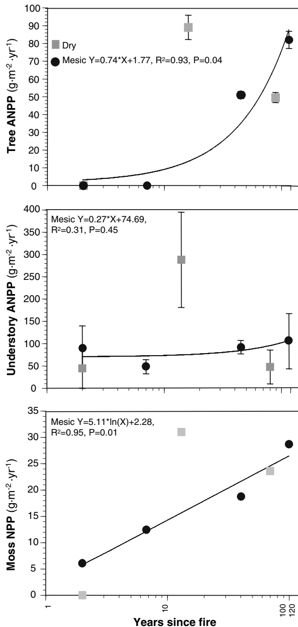
Figure 6. Tree, understory, and moss ANPP across dry and mesic chronosequences of sites near Delta Junction, Alaska, that differ in time since fire. Values are means ( \pm 1SE). Moss ANPP values are from Harden and others (In Review). Note that the x -axis is log-scaled to better visualize differences among younger sites.
