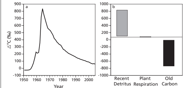
Figure 2. (a) Atmospheric content of radiocarbon in carbon dioxide during the bomb period. Radiocarbon ( \Delta^{14}\text{C} ) is expressed in units of permil (‰) compared to a pre-bomb material that is defined as having a value of zero. (b) Generalized values for possible respiration sources. The atmospheric value of +63\text{‰} for the year 2004 is depicted by the line on the graphs. Because radiocarbon in the atmosphere is currently declining, plant respiration is very close or slightly above current atmospheric values whereas detritus fixed over the past 50 years is enriched in radiocarbon up to +900\text{‰} . Old soil C ( >60 years) is the only source of C that could bring total ecosystem respiration below the atmospheric value.
