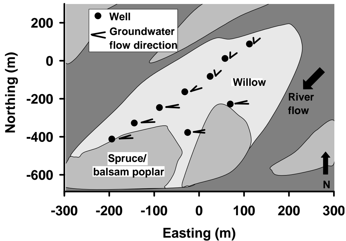
FIGURE. 7. Location of hyporheic wells (●) at Island II on the Tanana River. Arrows represent dominant flow vectors along subsurface flowpaths calculated from the change in hydraulic head in wells.
