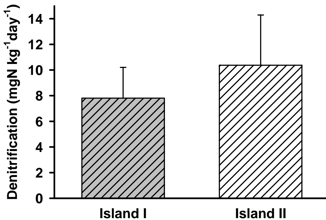
FIGURE. 9. Denitrification rates in hyporheic sediment (mean \pm SE) for Island I and II from July to September in 2005.
