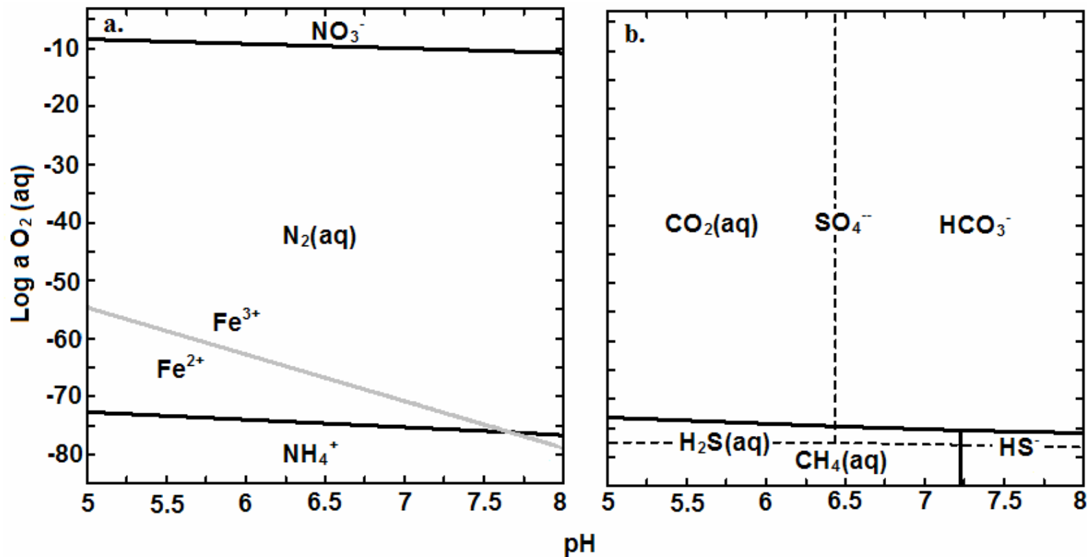
FIGURE. 3. Predicted thermodynamic equilibrium proportions of electron donors and acceptors as a function of the pH and oxygen activity ( \log a_{O_2} ) at 15°C, generated using Geochemist's Workbench 5.0. In deionized water, the activity of oxygen is equal to the concentration of oxygen ( \text{mol L}^{-1} ). Nitrogen is the black line and iron is the grey line (panel a). Sulfur is the black line and carbon is the dashed line (panel b).
