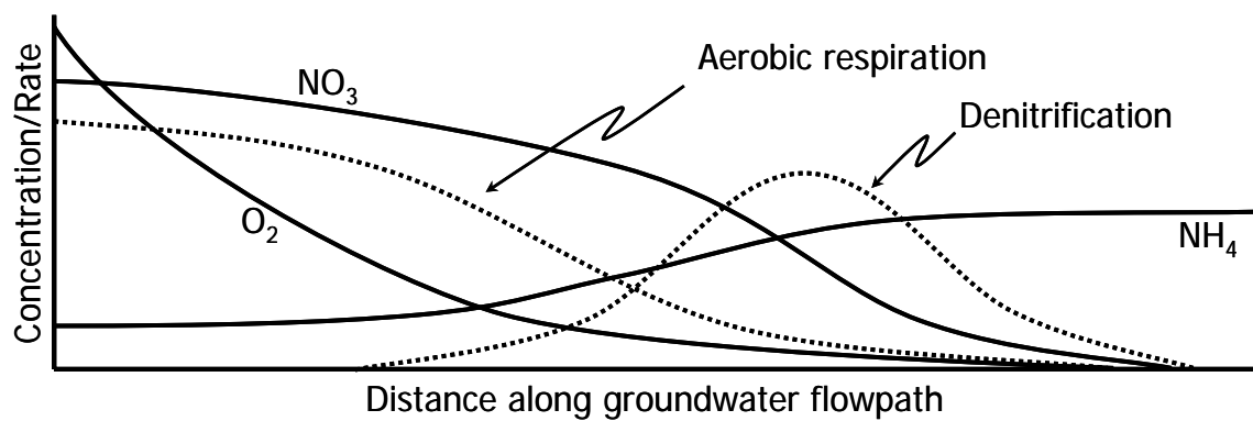
FIGURE. 2. Conceptual model of metabolic processes along subsurface flowpaths from Jones (1994).
