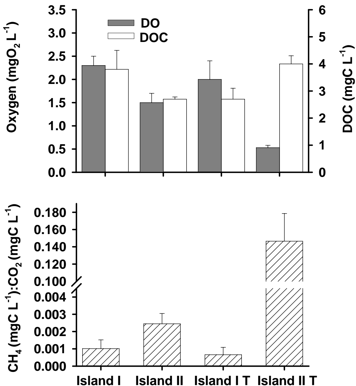
FIGURE. 6. Concentrations of hyporheic oxygen and dissolved organic carbon (mean \pm SE; panel a), and indices of hyporheic anaerobiosis ( \text{CH}_4:\text{CO}_2 ; mean \pm SE) for the well transects (Island I and II) and wells at the willow-alder transitional wells (Island I T and Island II T; panel b).
