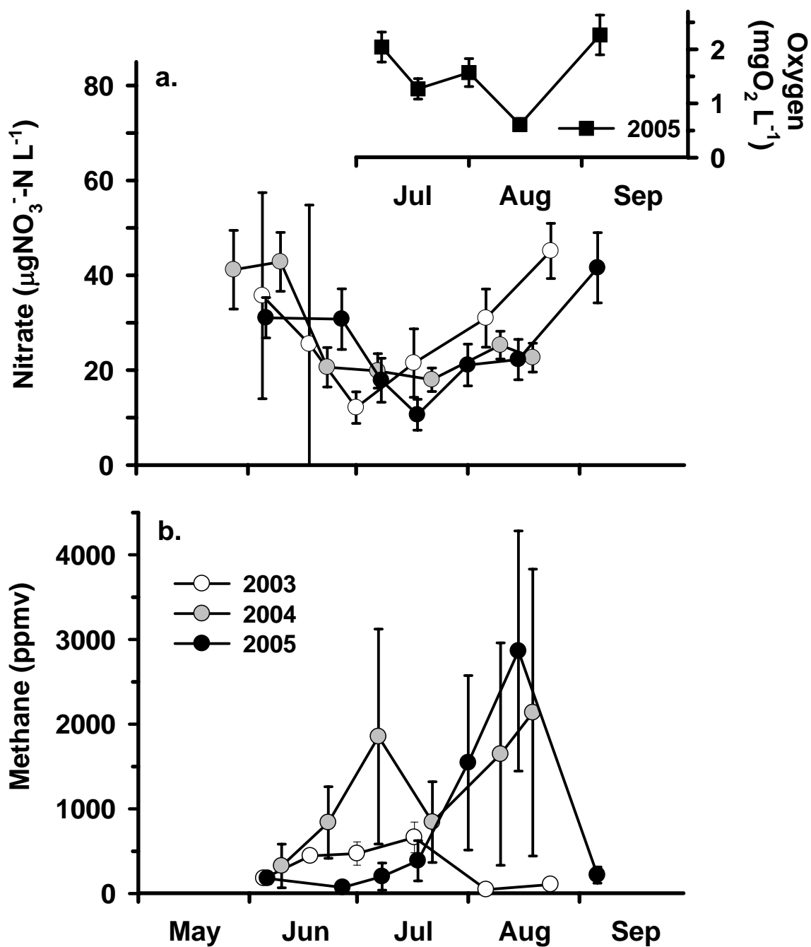
FIGURE. 10. Temporal variations in hyporheic nitrate concentration (mean \pm SE; panel a) and methane partial pressure (mean \pm SE; panel b) at Island II over the three study years.
