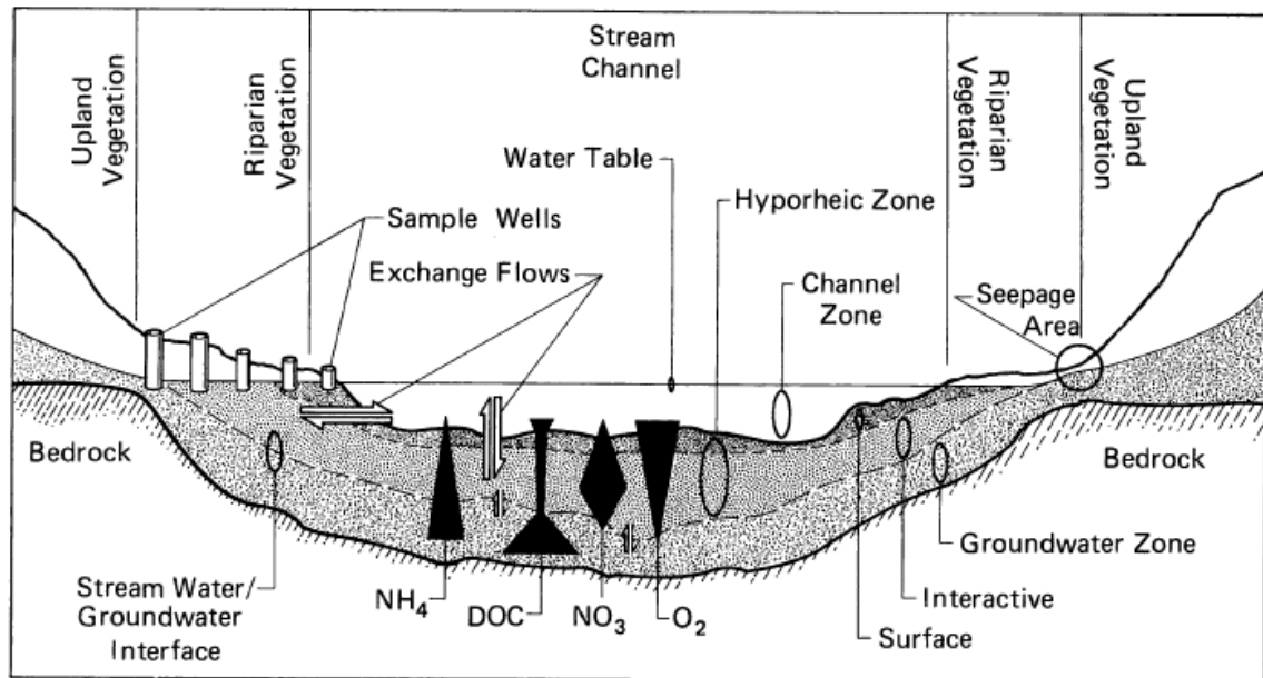
FIGURE. 1. Conceptual model of the groundwater-surface water interface from Triska et al. (1989). Waters are divided into three zones: a channel zone containing surface water, a hyporheic zone, and a groundwater zone. The hyporheic zone is characterized by chemical gradients in \text{NH}_4^+ , \text{O}_2 , DOC, \text{NO}_3^- .
