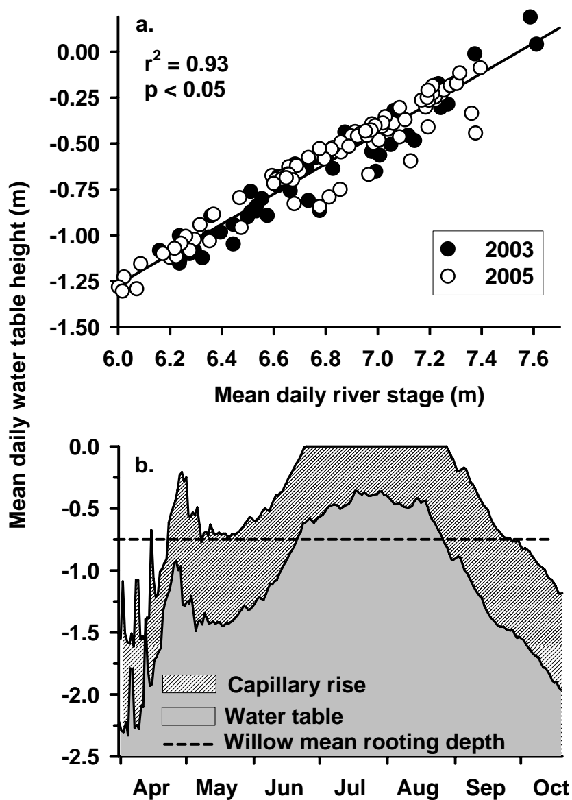
FIGURE. 8. Relationship between mean water table height and mean daily river stage (panel a) for both islands. Line indicates statistically significant regression at p < 0.05 and r^2 = 0.93 , Slope = 0.82 and y = 0.8227x + -6.2044 . Predicted mean water table height using the regression relationship in panel a and river stage data (mean river stage from 1990 - 2005) from Fairbanks USGS gauging station (panel b). Dashed horizontal line denotes mean willow rooting depth.
