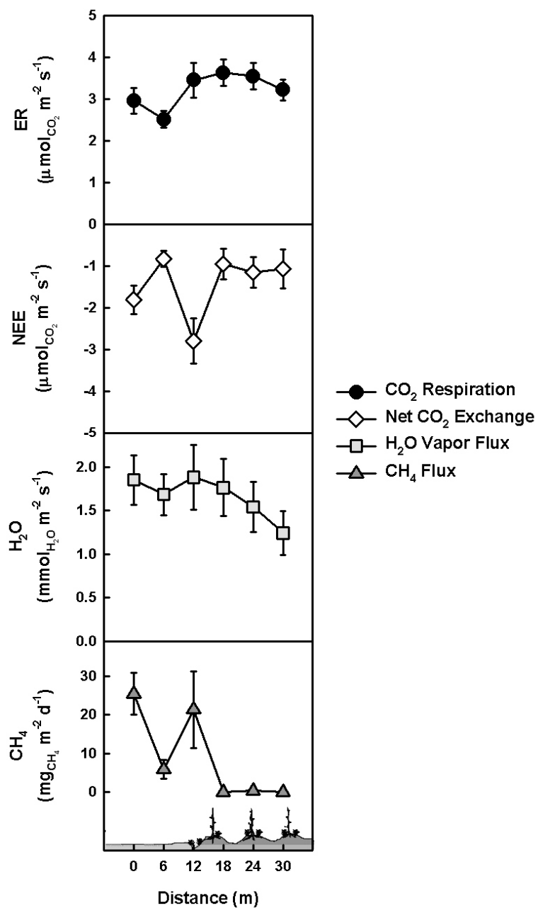
Figure 4. Mean fluxes across the transect. Mean ecosystem respiration, NEE, water and CH 4 fluxes across the transect for the growing season of 2004 (error bars = \pm SE, n = 16 for CO 2 , NEE and H 2 O and n = 13 for CH 4 ). Carbon uptake is denoted with negative numbers and carbon emissions with positive numbers.
