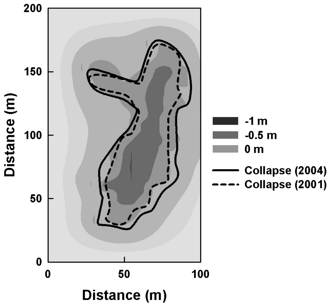
Figure 3. The expansion of the collapse bog. A survey of the extent and depth of the collapse. The dashed line is the margin of the collapse in 2001 and the solid line in 2004. Gradients indicate collapse depth (m).
