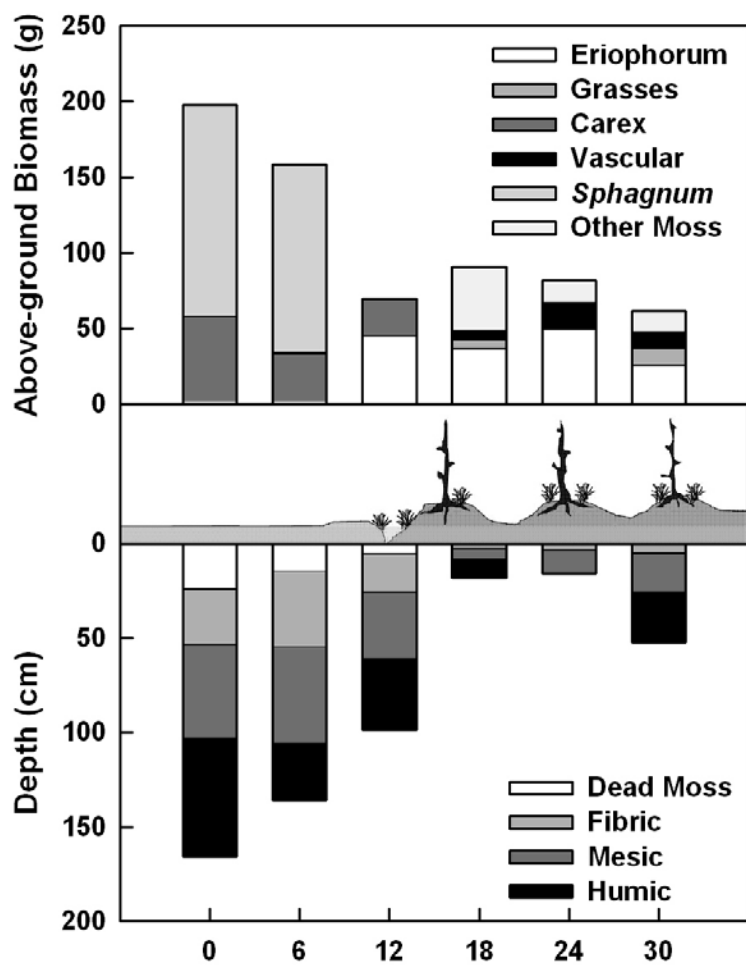
Figure 2. Biomass and soils across the transect. Mean above-ground biomass ( \text{g m}^{-2} , n = 2 ) and mean measured soil horizon depths described using the Canadian Soil Classification system (cm, n = 2 ).
