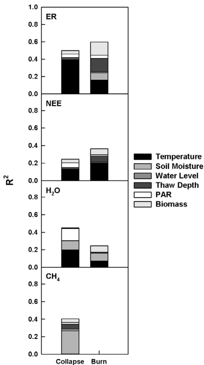
Figure 5. Multiple linear regression r^2 values for all significant parameters. The proportion of variation explained each significant model parameter for multiple linear regression models of all fluxes for the collapse and burn portions of the landscape. All models are significant at p < 0.05 except for the H 2 O burn model, which was marginally significant ( p = 0.08 ).
